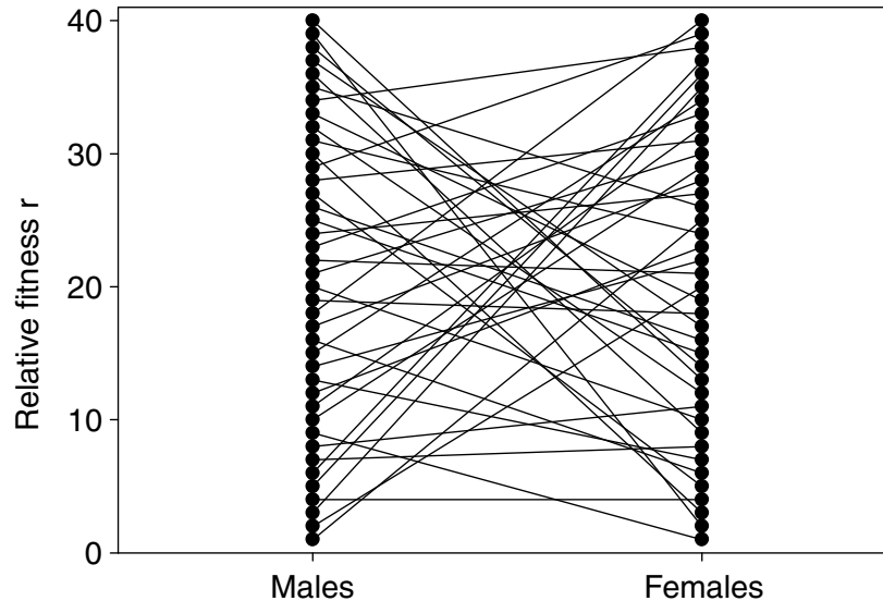
Figure 1.3. Plot of male and female adult fitness in a suite of discrete Drosophila melanogaster haplotypes. Note that these haplotypes tend to have opposing effect on fitness in the two sexes: haplotypes that result in high fitness in males tend to result in low fitness in females. These data demonstrate that, for at least some genes in this species, their effect on the fitness of males and females is antagonistic. (Reprinted from Chippindale et al. 2001, with permission from the National Academy of Sciences.)
