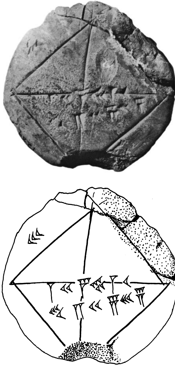
Figure 1.1. YBC 7289
